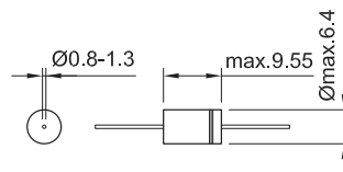
Abmessungen Bypassdiode (mm) Dimensions of bypass diode (mm)
